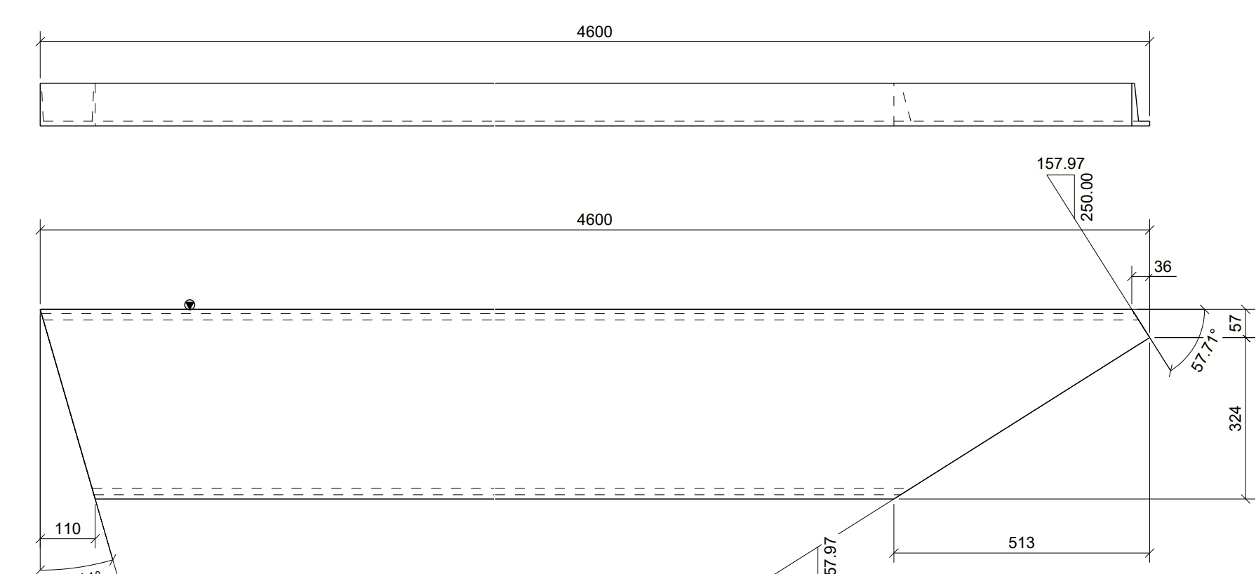
DETAIL OF 3S1004
