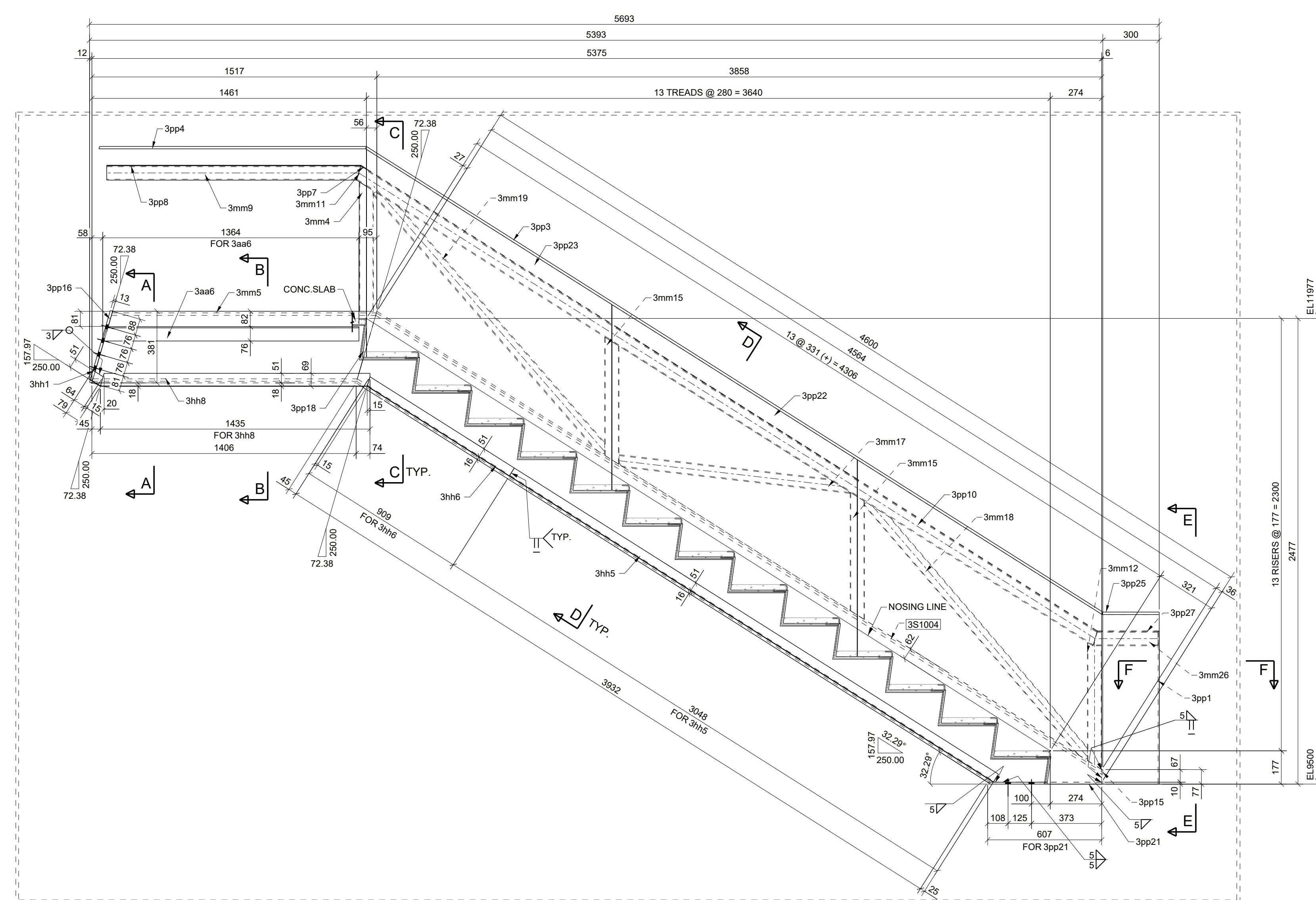
DET. 2 STRINGER WITH PANEL DET. 1 STRINGER WITH FRAME
