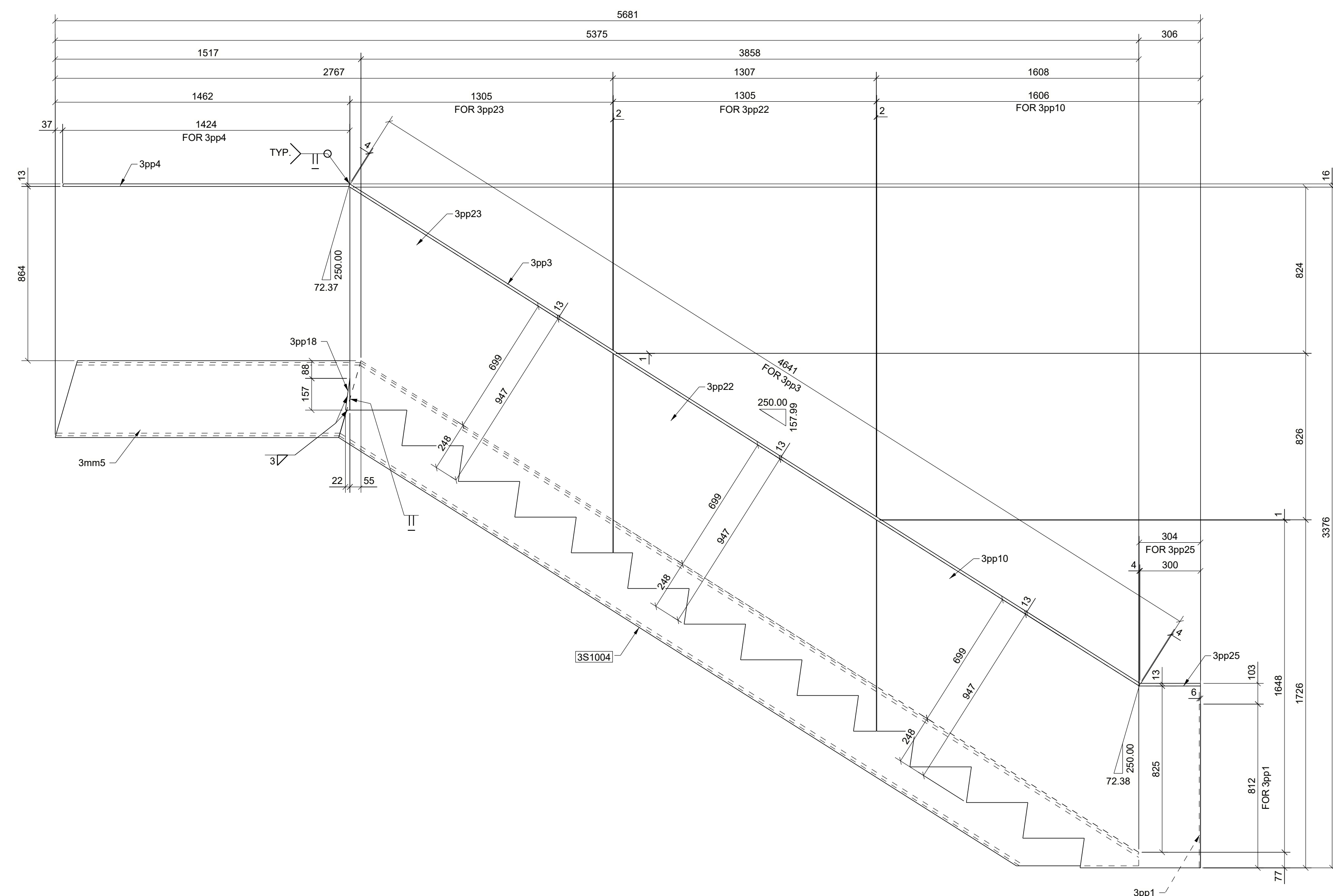
DETAIL-2 STRINGER WITH PANEL
