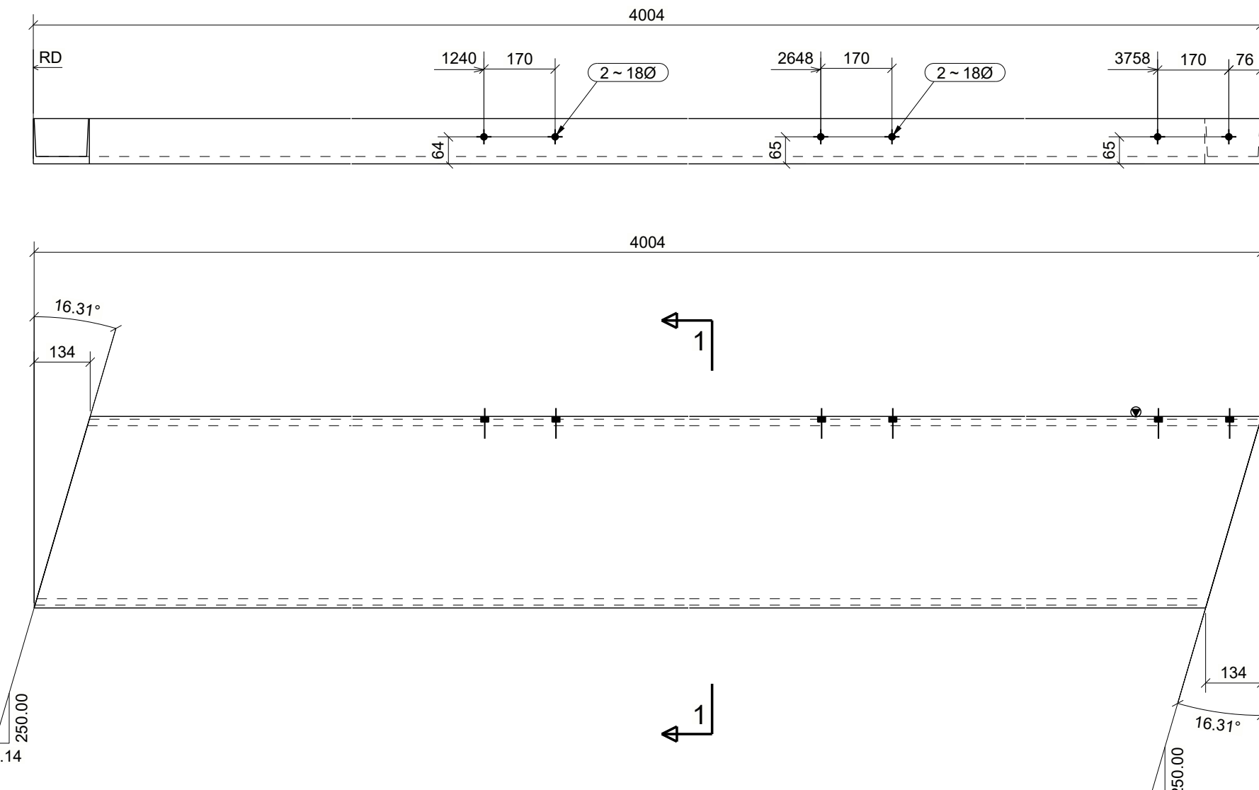
DETAIL OF S4S1003
