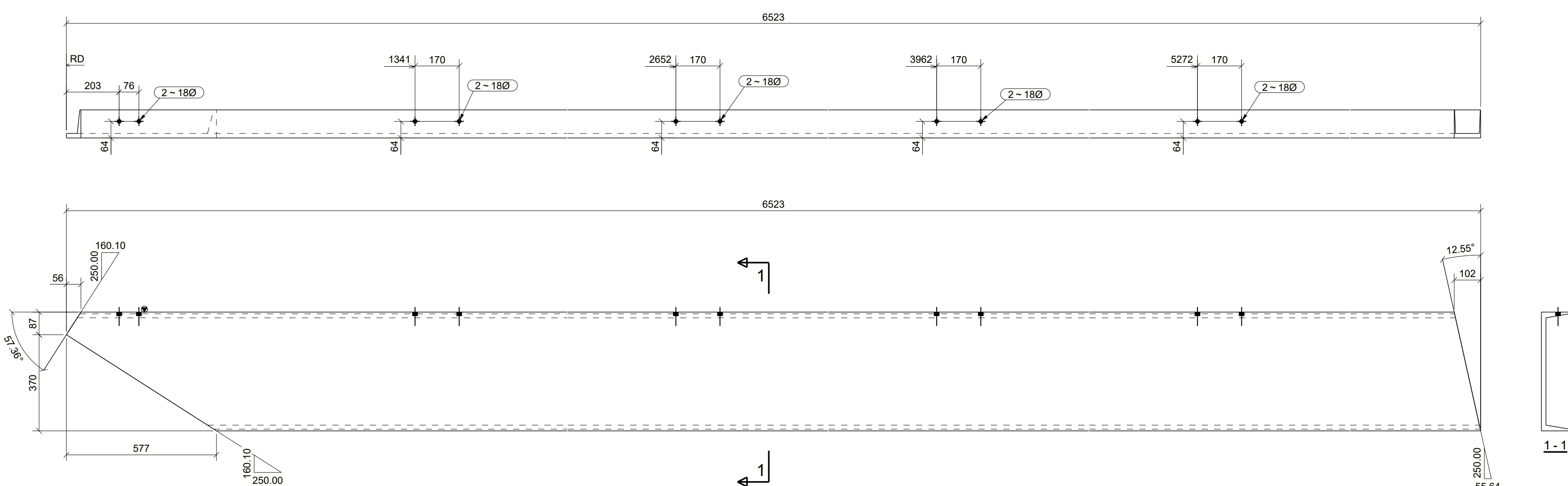
DETAIL OF 54S1001
