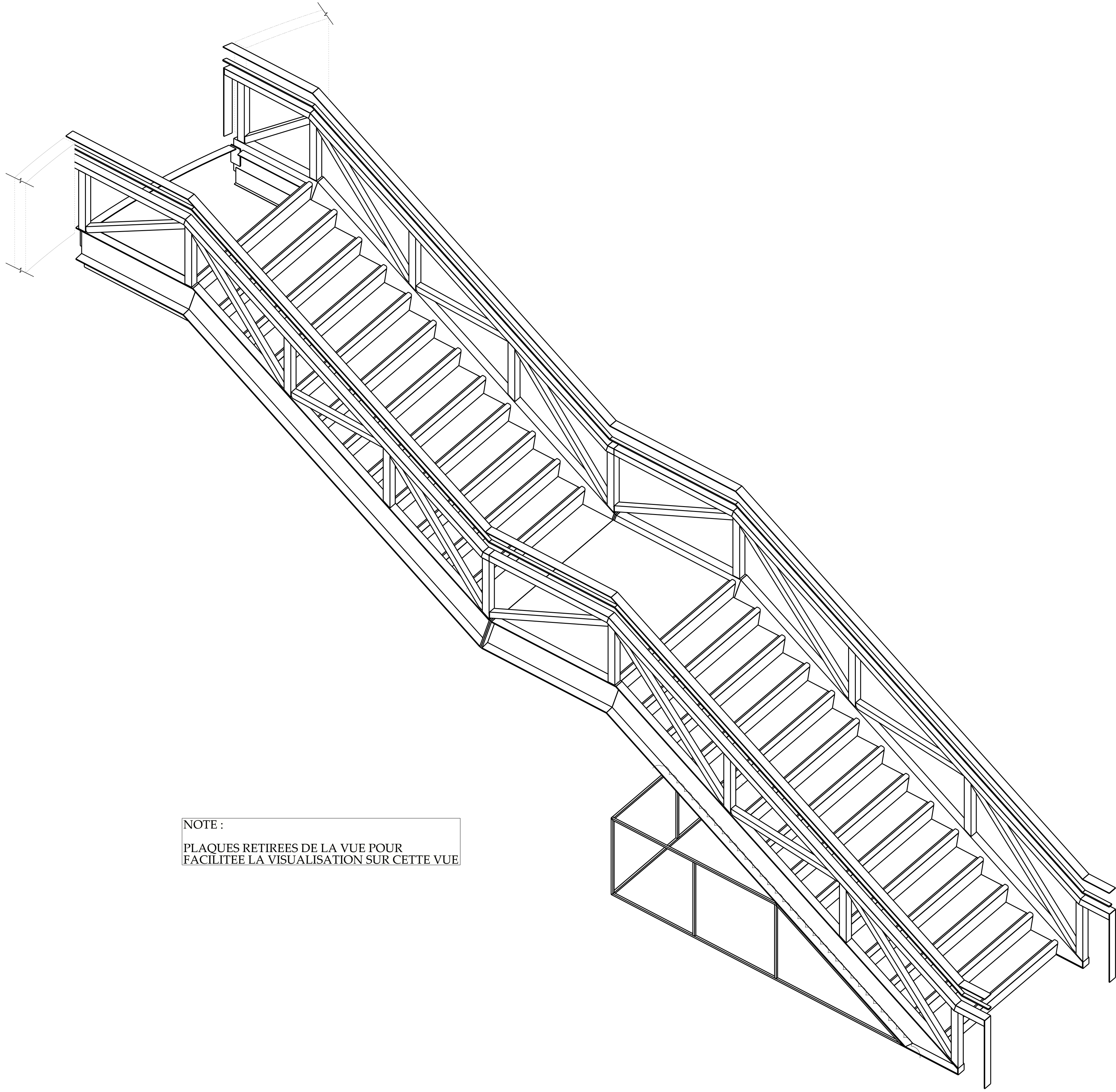
3D - VIEW WITHOUT RAIL PANELS
